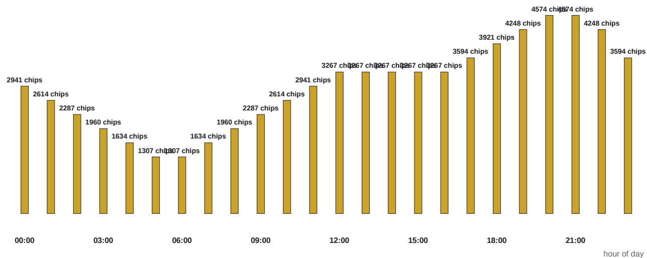
Handle per hour - standard day, 100-chip ante
