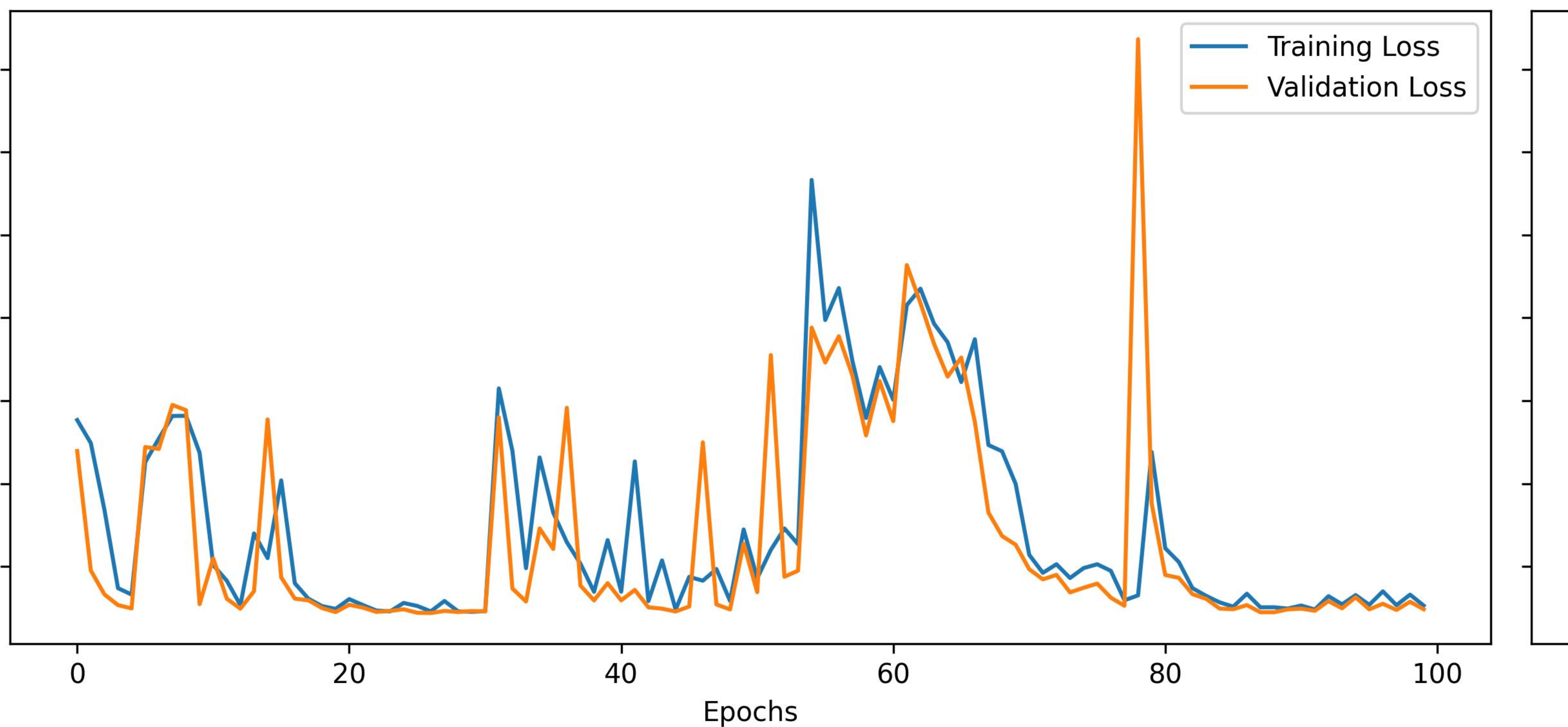
LSTM
