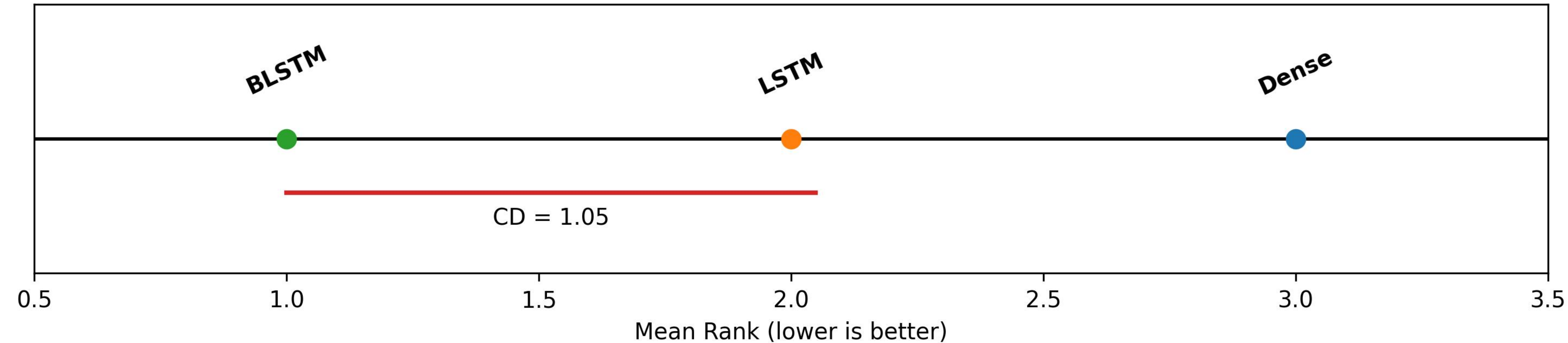
Critical Difference Diagram (MAE)
