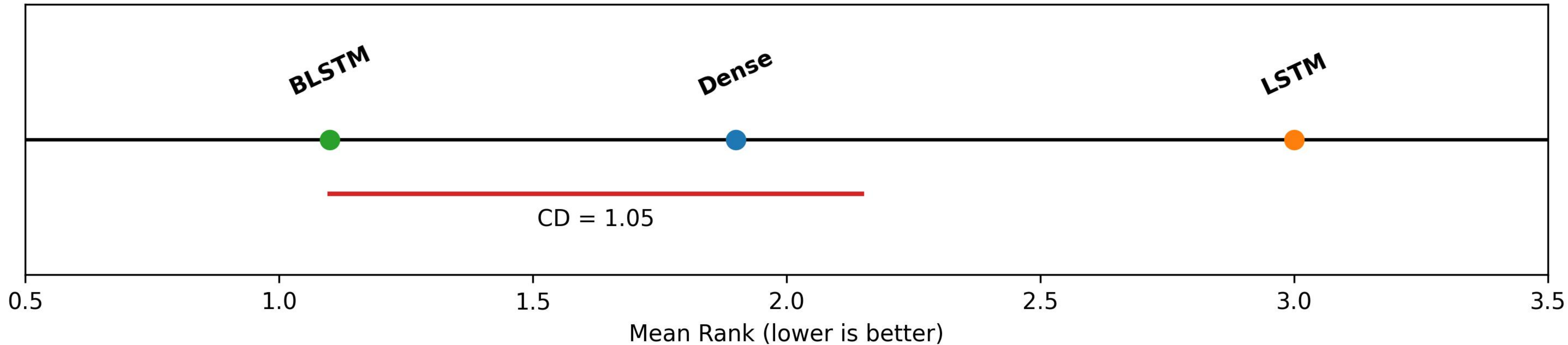
Critical Difference Diagram (MAPE2)
