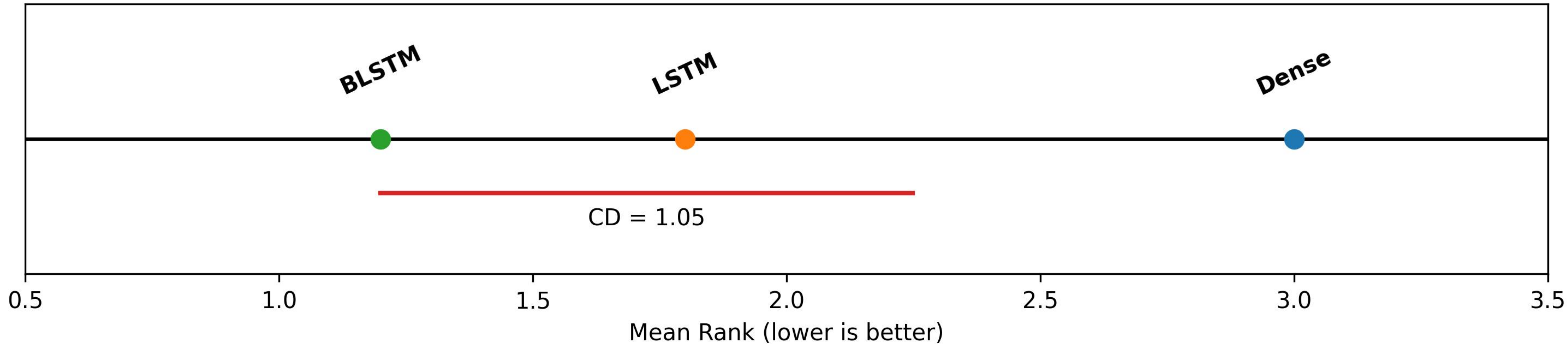
Critical Difference Diagram (MSE)
