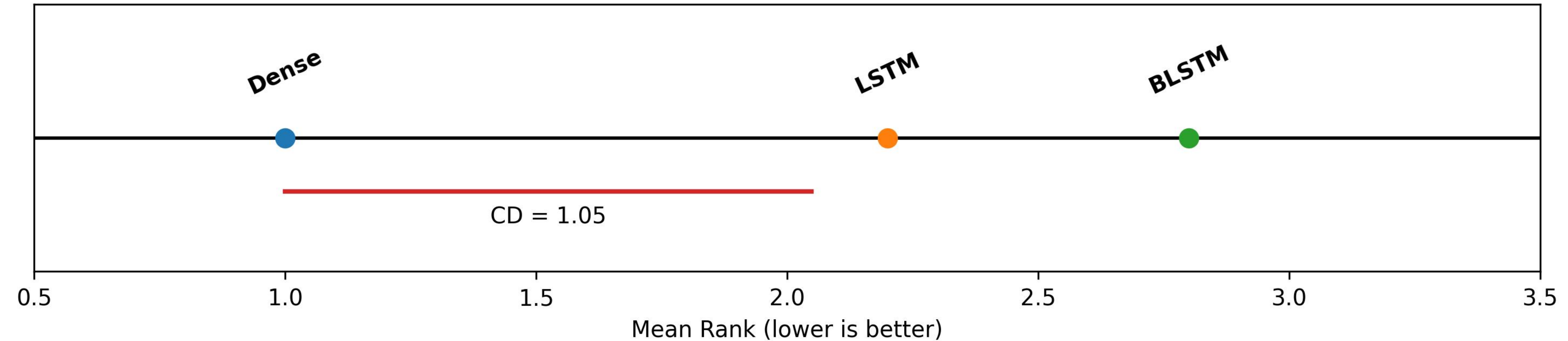
Critical Difference Diagram (R2)
