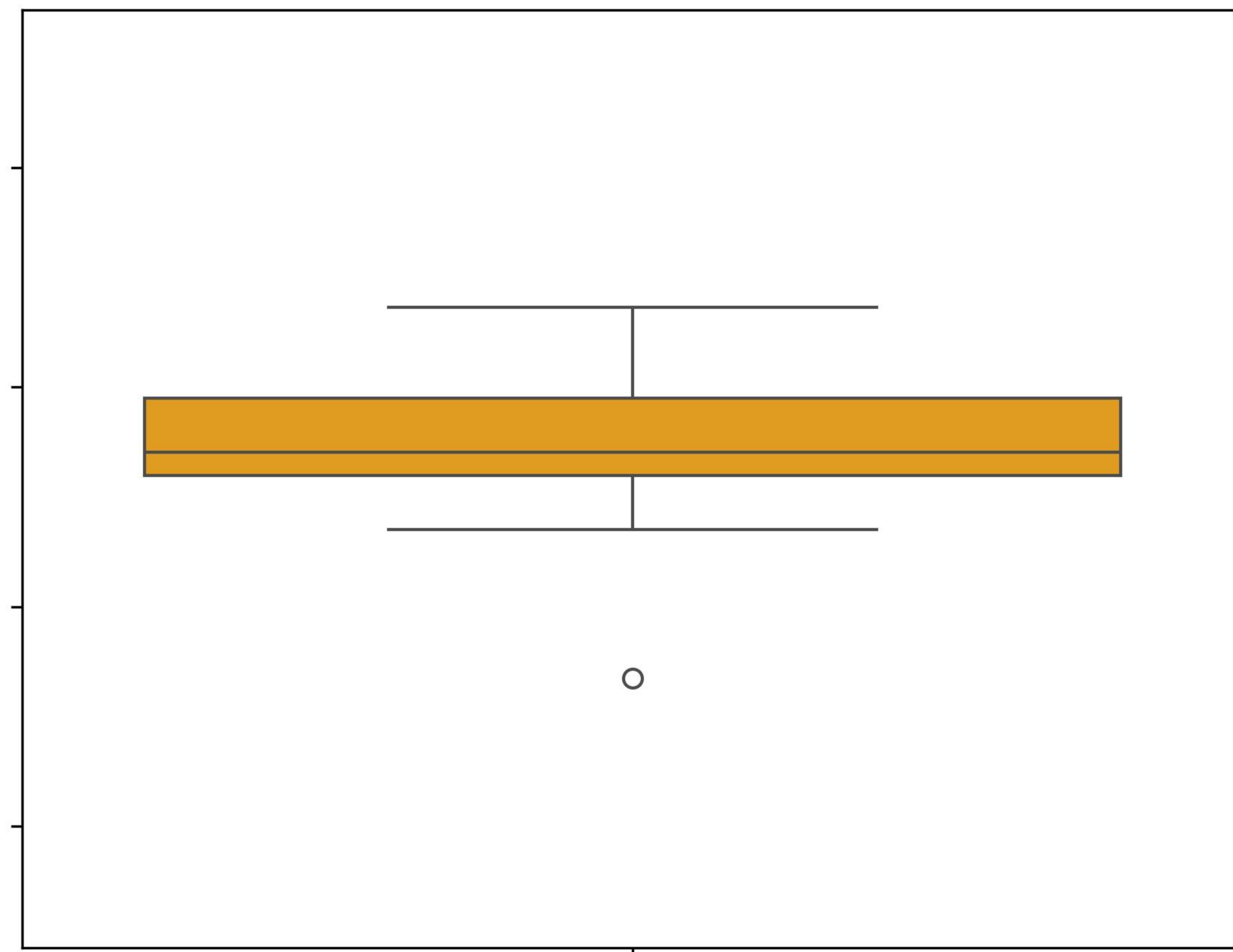
LSTM
