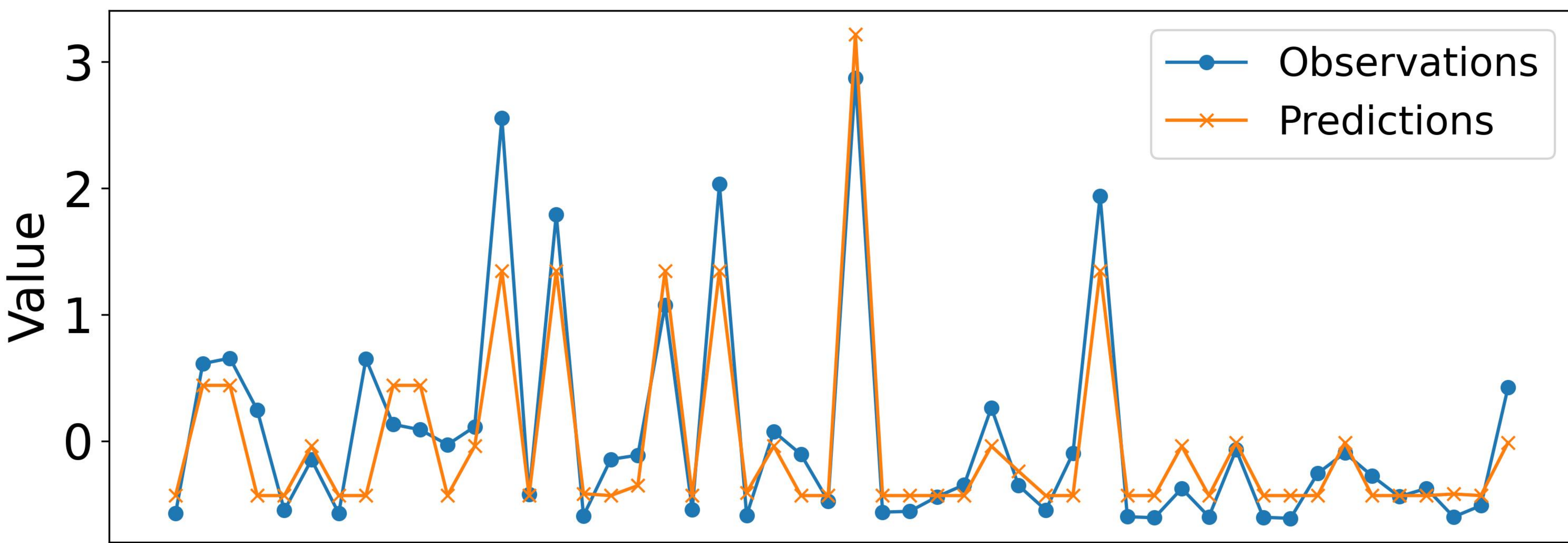
LSTM
