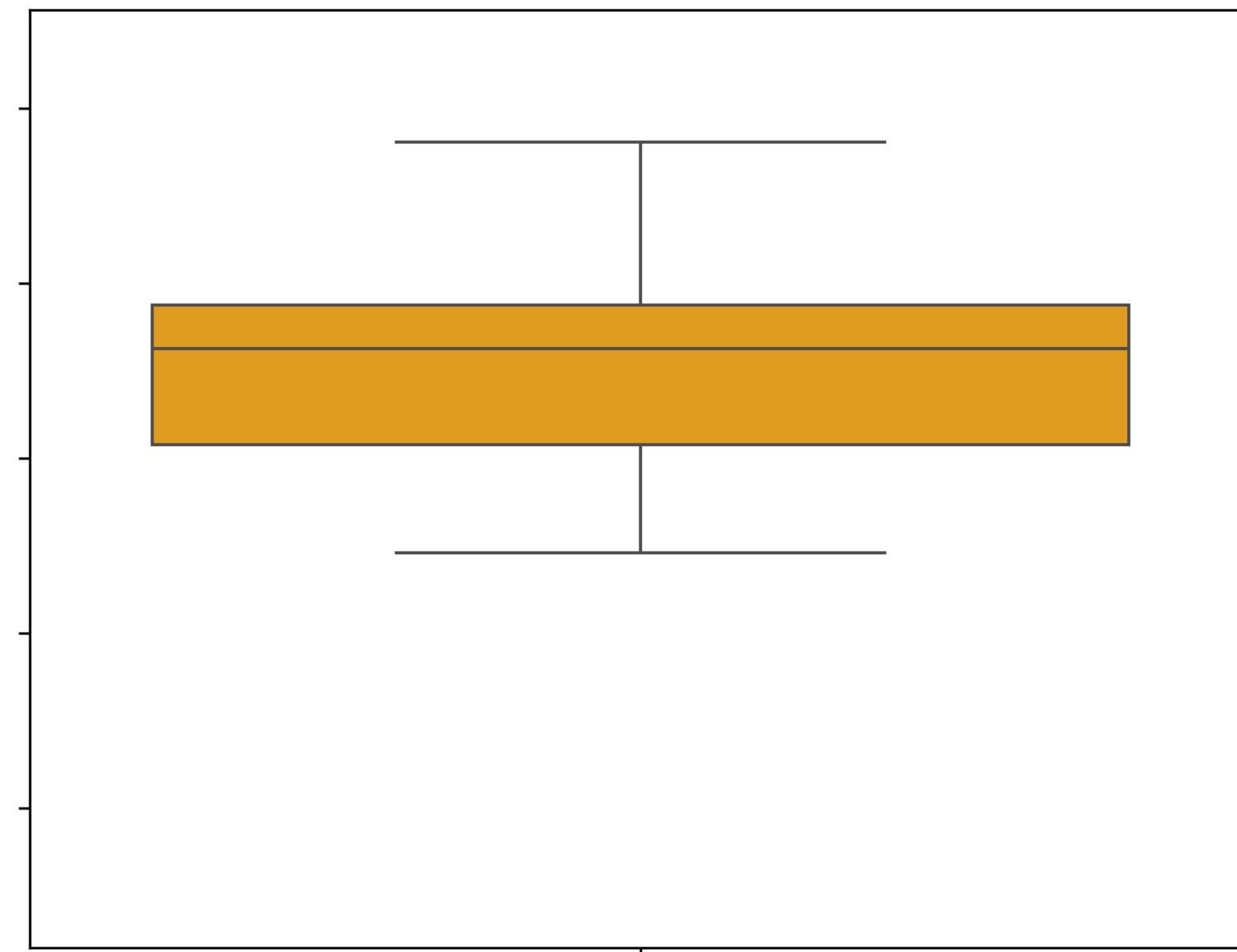
LSTM
