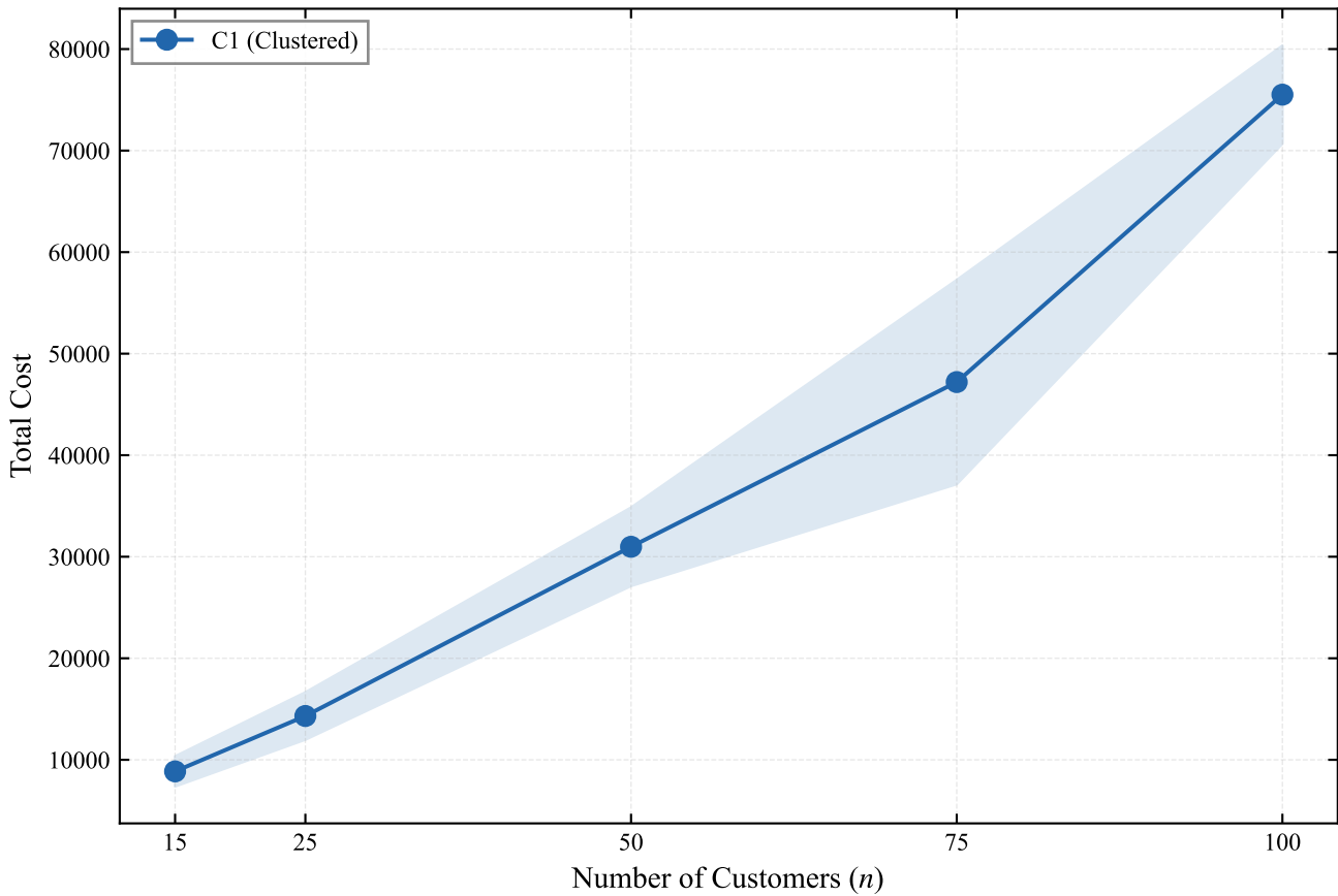
(a) Total Cost vs. Number of Customers
