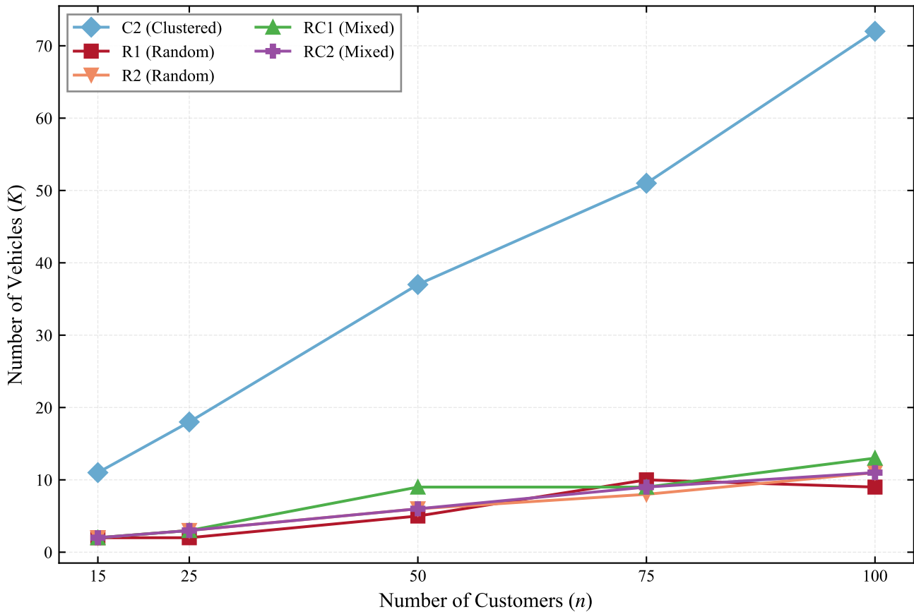
(c) Number of Vehicles vs. Number of Customers
