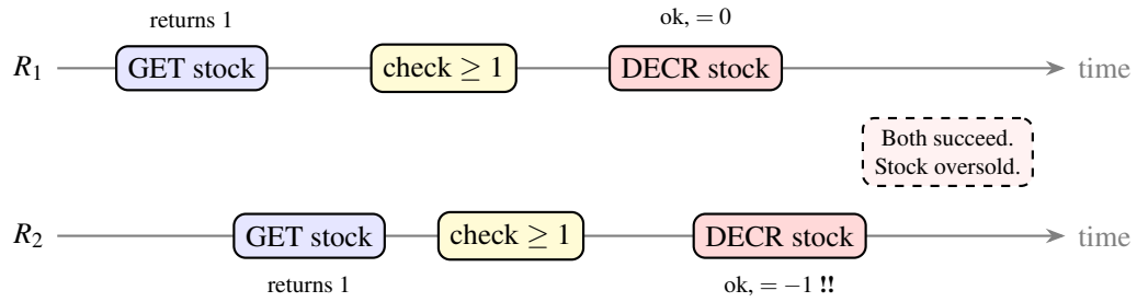
Figure 5.1: Lost-update race on a single-resource decrement. R_1 and R_2 each read stock=1 from the cache (or from Redis without an atomic guard), each independently passes the availability check, and each issues a successful decrement — leaving the backend in an inconsistent stock=-1 state.
