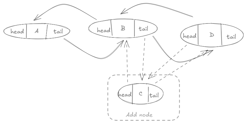
LinkedList
