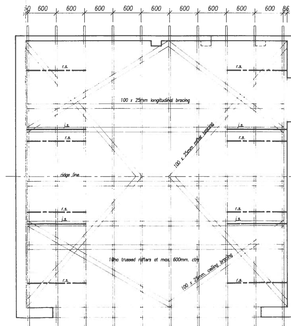
ROOF CARCCASING PLAN
