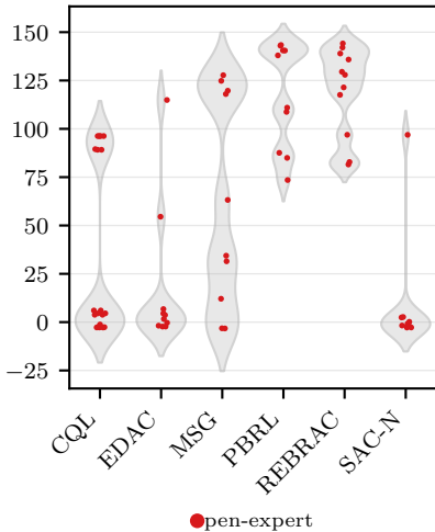
D4RL Normalized Score
