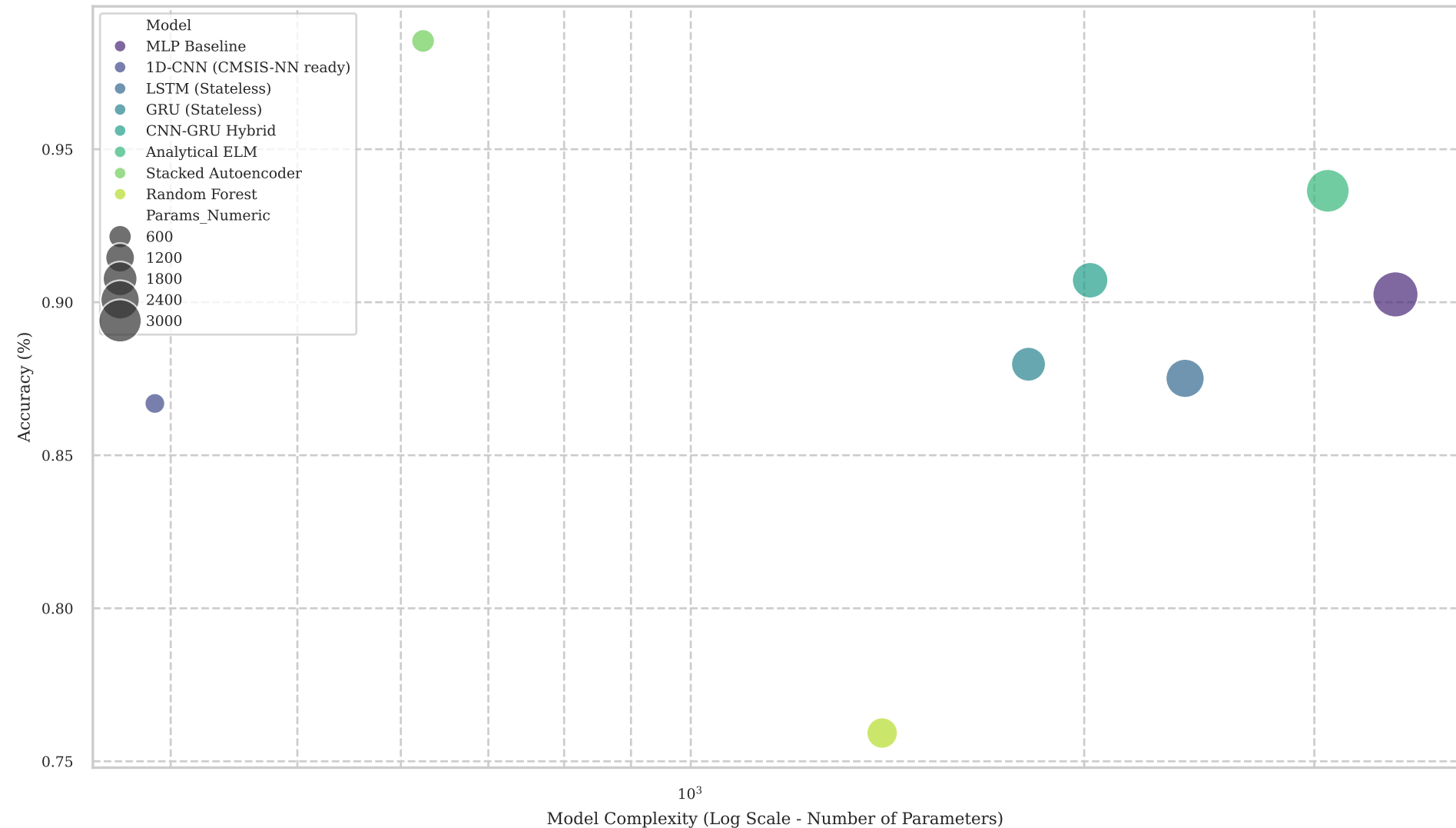
Accuracy vs. Computational Complexity Trade-off
