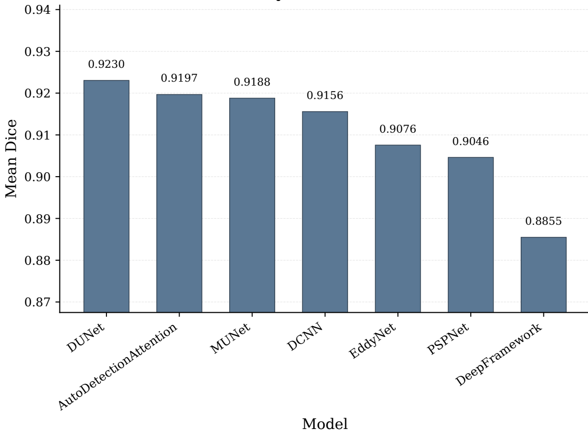
Mean Dice on SCSE-Eddy
