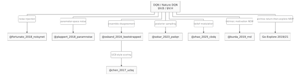
Fig. 3. Genealogy of brittle-exploration methods (§IV.C).
