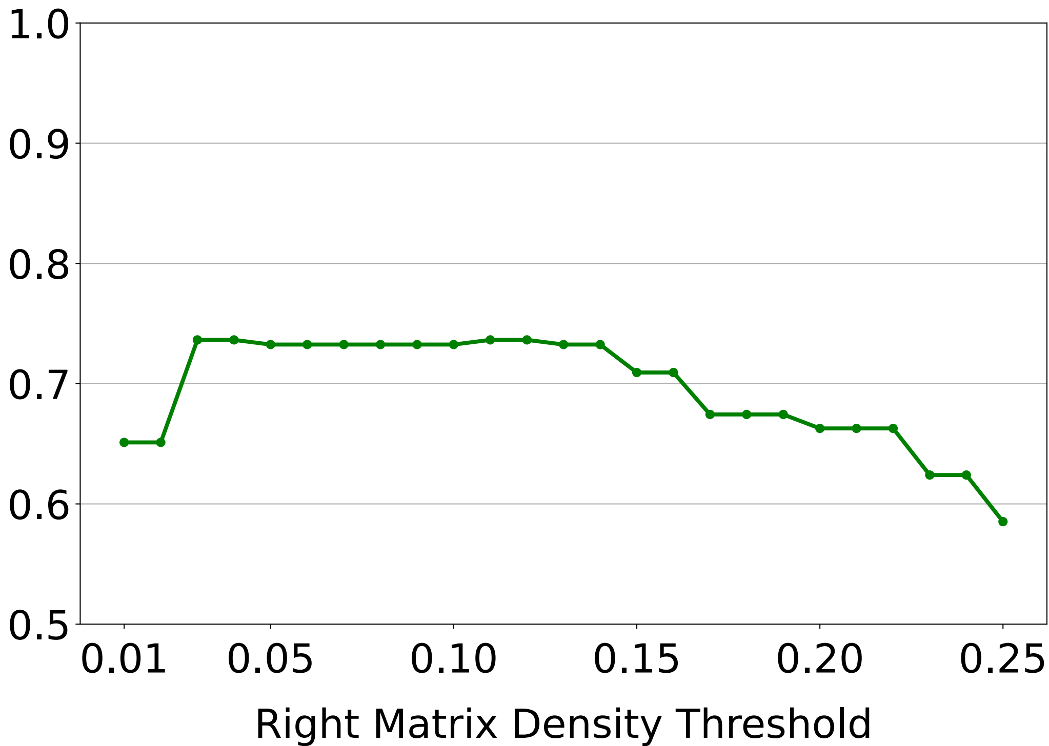
Accuracy
