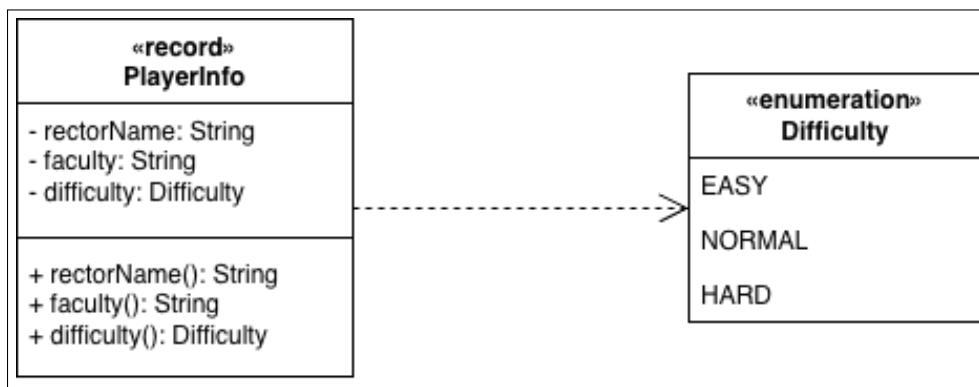
Figura 2.10: Value Object PlayerInfo come Java record.
