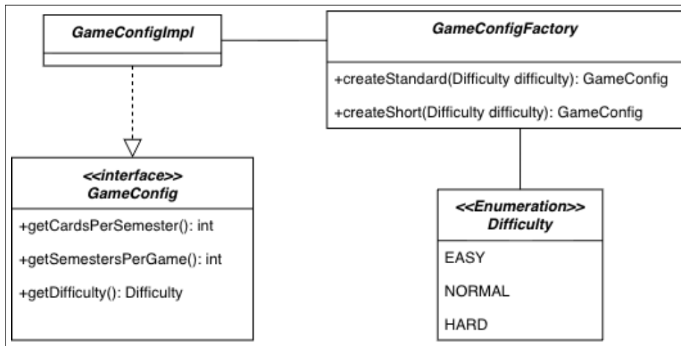
Figura 2.11: Pattern Static Factory Method in GameConfigFactory
