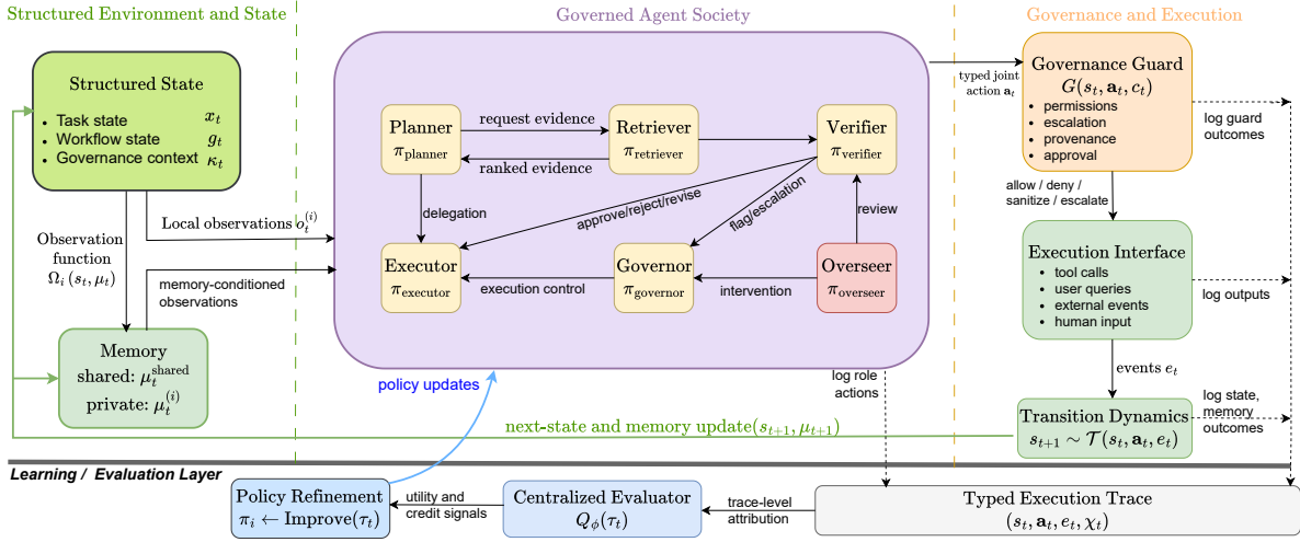
Fig. 1. Runtime and evaluation architecture of a governed agent society. Roles observe structured state and memory, propose typed actions, and high-impact proposals pass through the guard before reaching tools, people or the public. Every proposal produces one trace record. [TODO: relabel the boxes with the MAPE-K terms and add the evidence store to the state box.]
