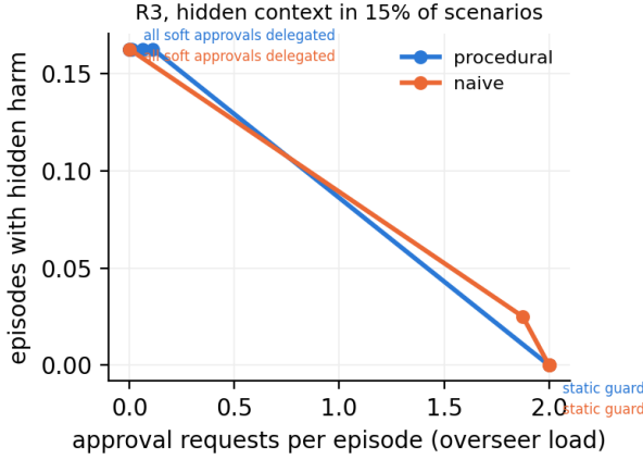
Fig. 3. Overseer load against hidden harm for static and trust-adaptive governance, rule set R3, hidden context in 15% of scenarios. Points on each line are thresholds 0.9, 0.7, 0.5, 0.3 and 0.0 from right to left; for the procedural roles the four lowest coincide.
