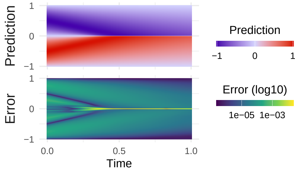
1D Burgers' Equation
