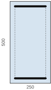
Section 250×500 215 barres
