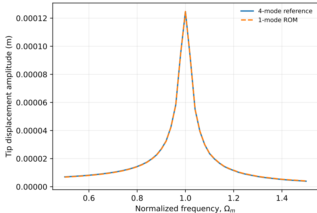
(a) Structural ROM validation
