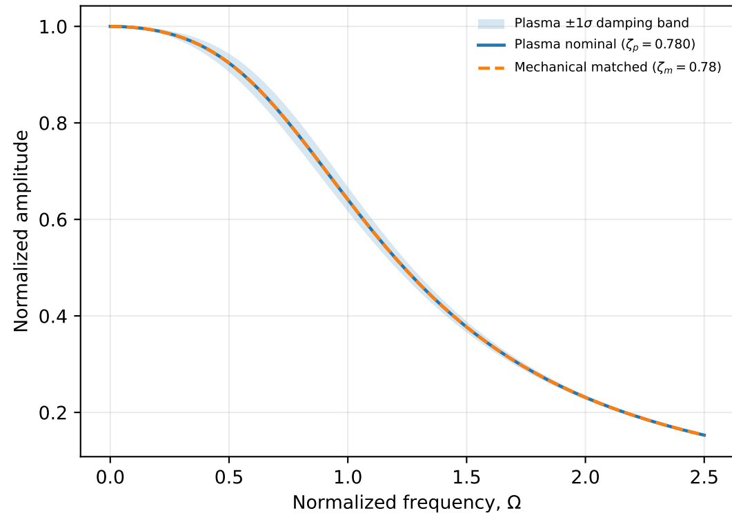
(a) Damping-matched amplitude response
