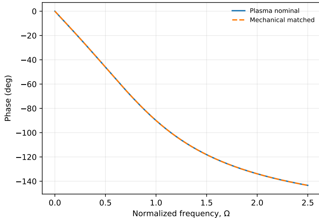
(b) Damping-matched phase response
