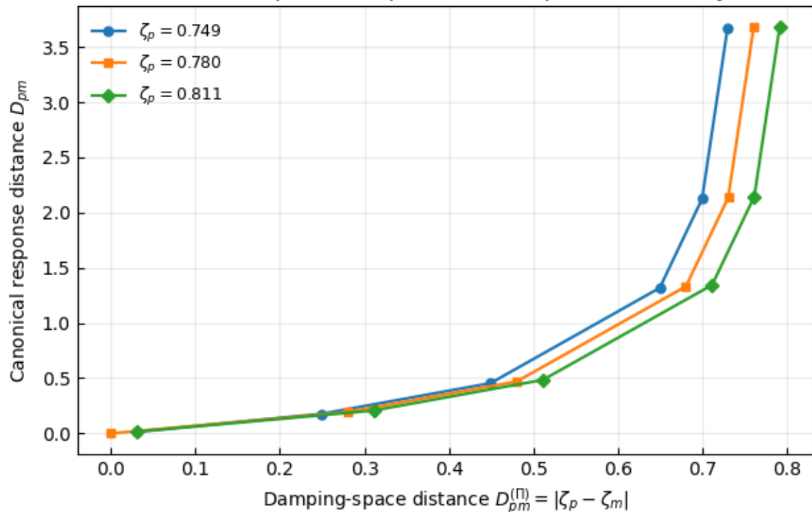
Canonical pole-level parameter-response sensitivity
