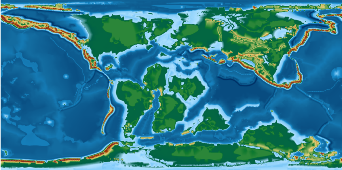
Figure 3: 100Ma map from PANALESIS (2026) at 0.1 \times 0.1^\circ resolution
