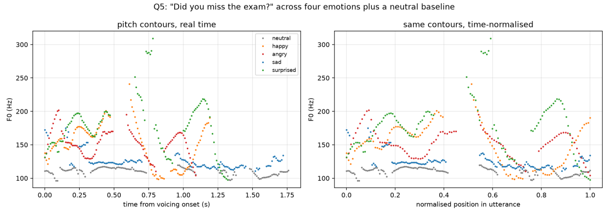
Figure 7: Pitch contours, in real time and time-normalised
