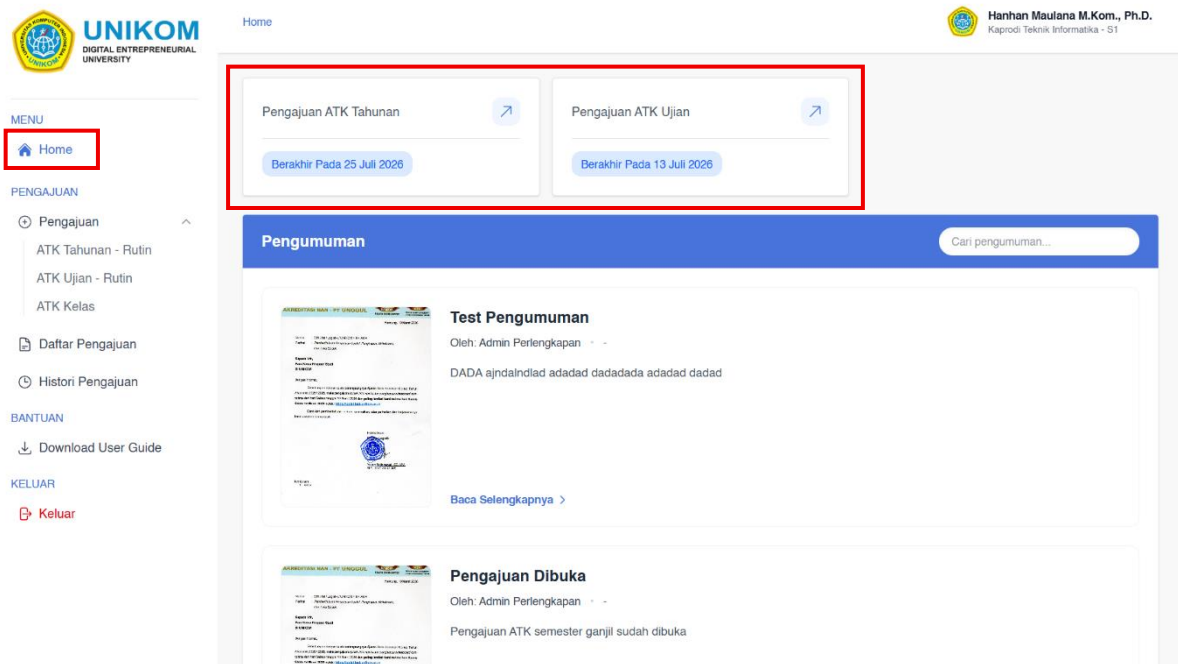
Gambar 2 Halaman Home(1)
