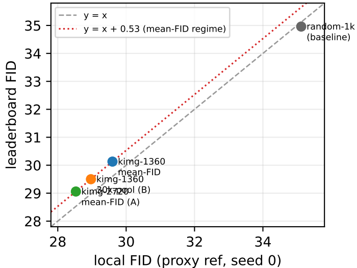
(a) FID is predictable: +0.53 offset
