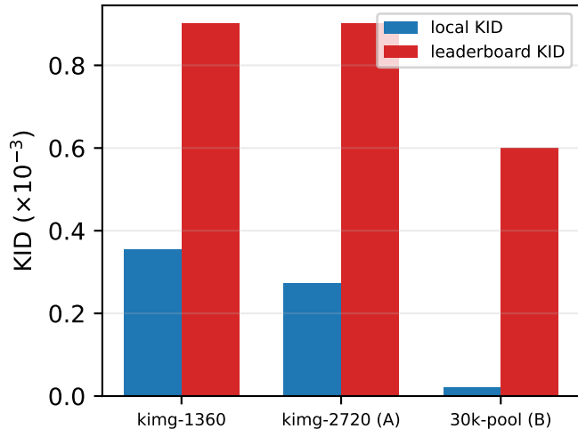
(b) KID is over-optimistic locally
