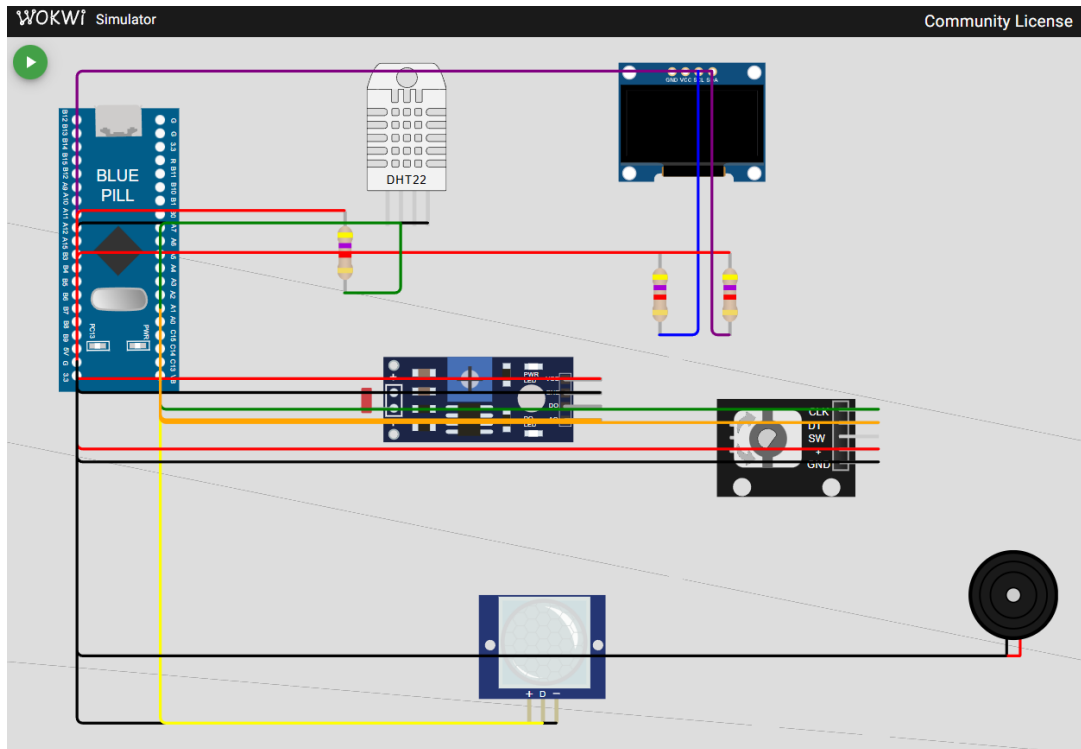
Figure 1. User-supplied circuit capture: all sensing, input, display, and alarm components share the Blue Pill and common ground.
