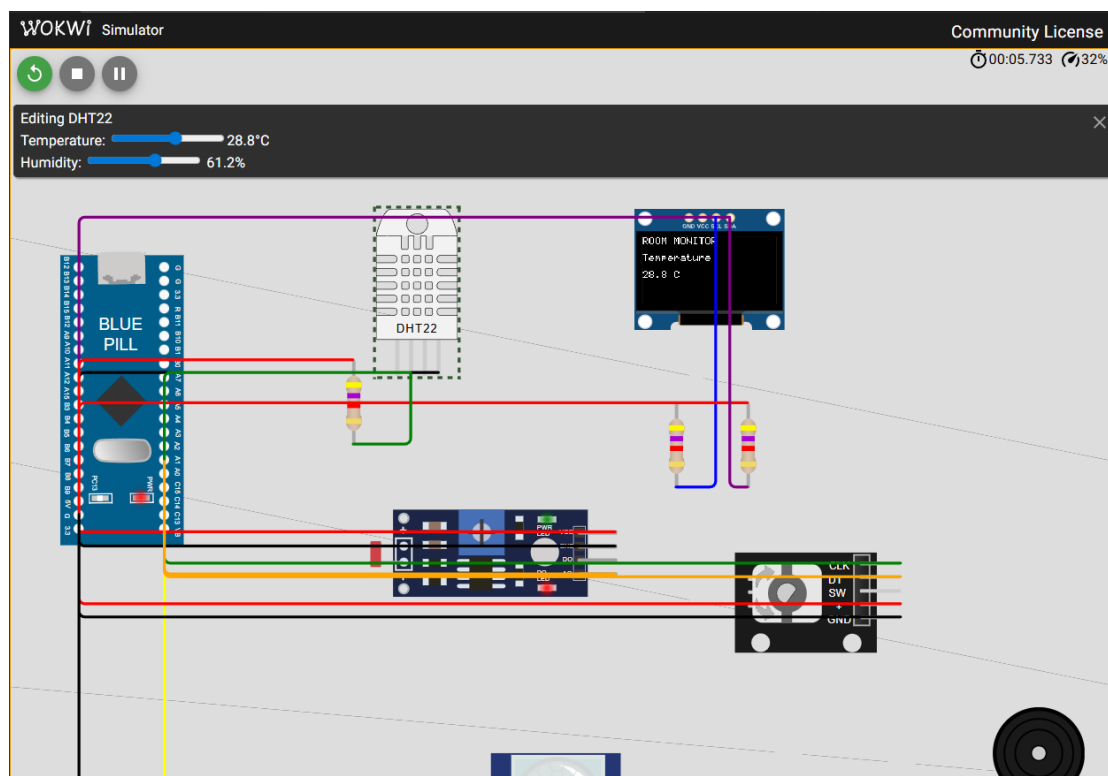
Figure 2. Actual user capture at 5.733 simulated seconds. The DHT22 control and OLED both show 28.8 C; the humidity control is 61.2 percent. The terminal is not visible, so no simultaneous UART measurement is claimed.
