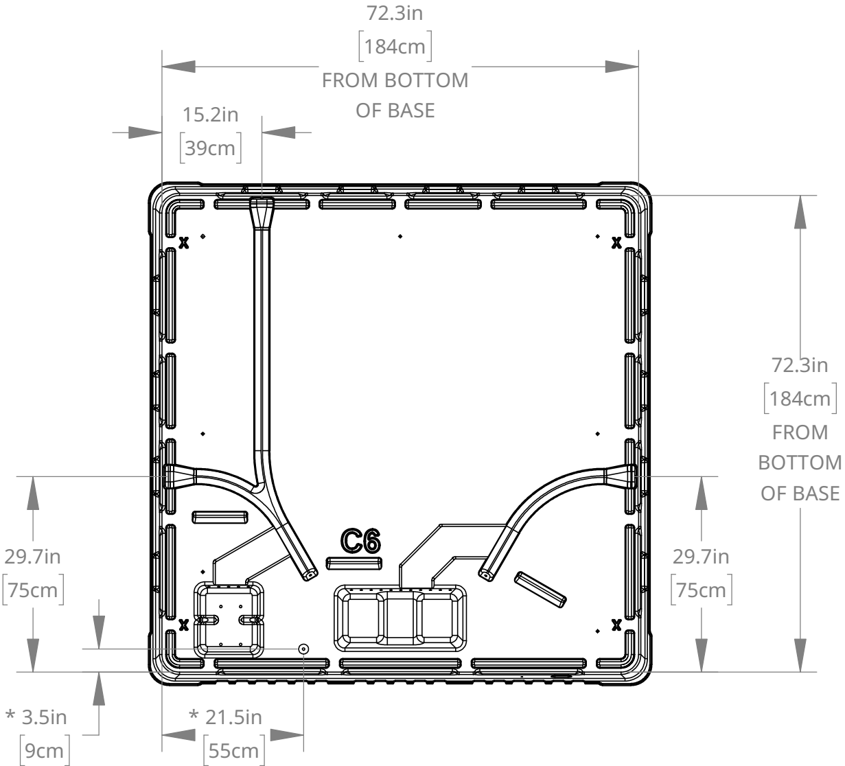
BASE VIEW
