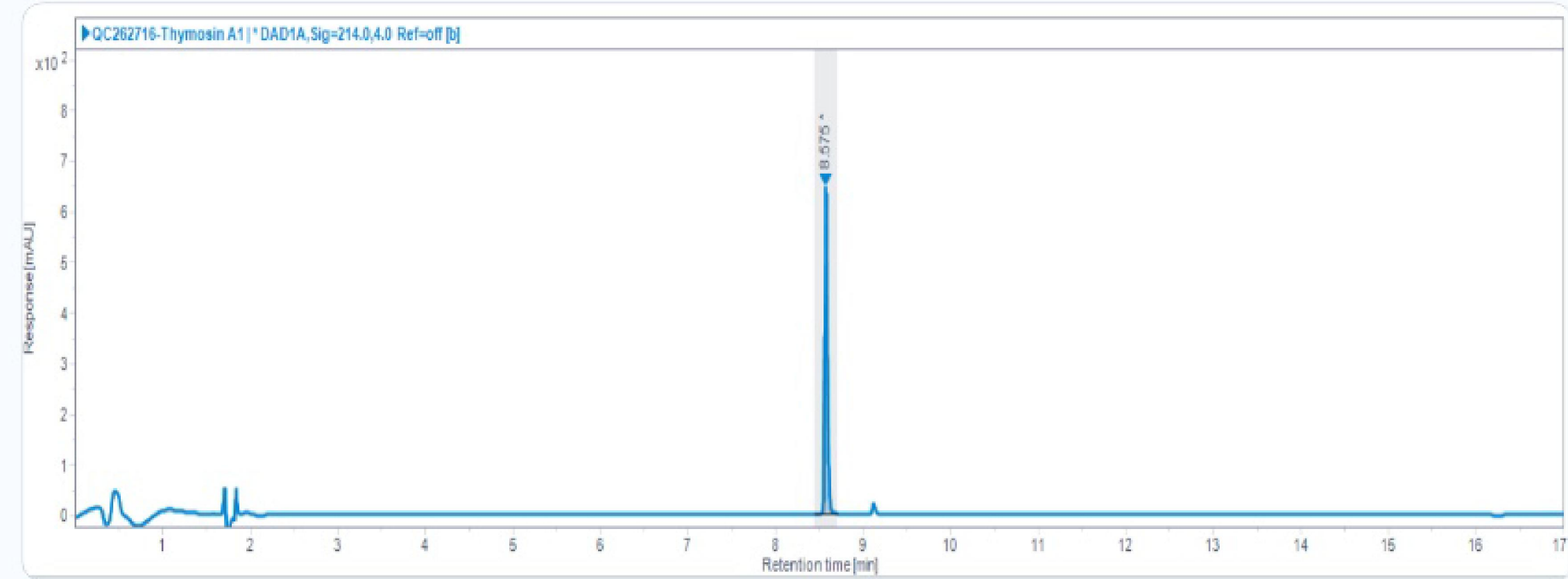
HPLC Chromatogram (Retention Time: 8.575 min)
