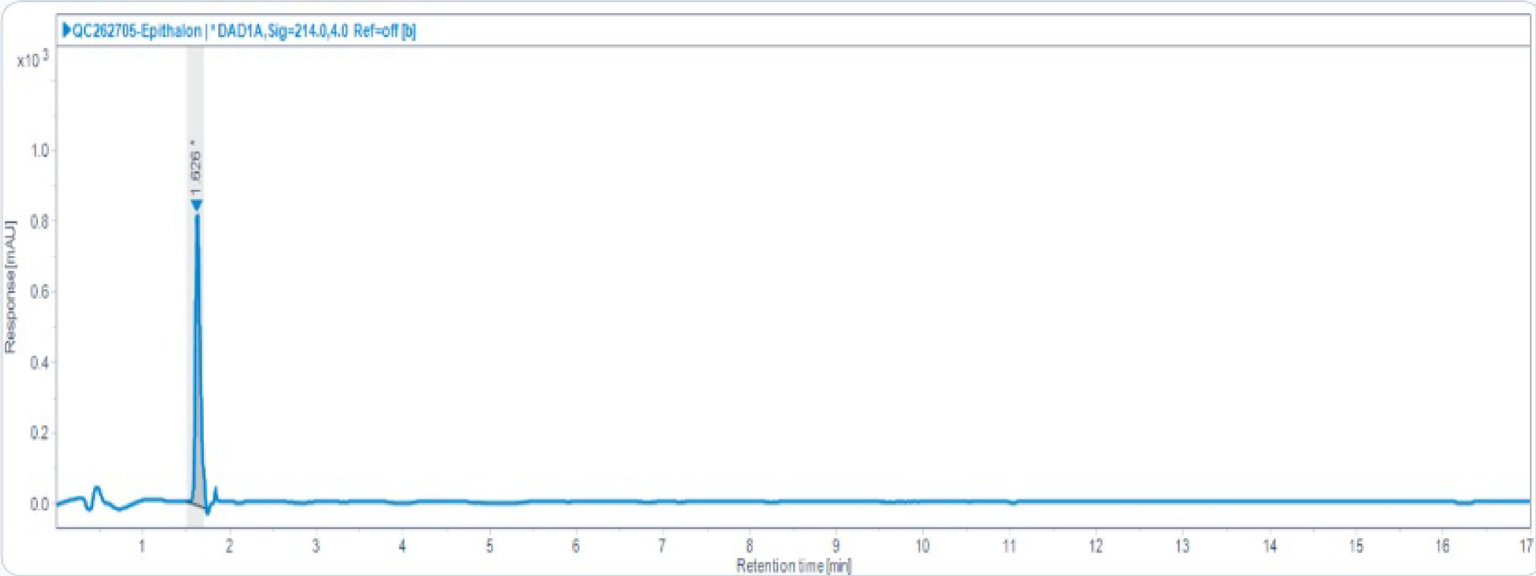
HPLC Chromatogram (Retention Time: 1.626 min)
