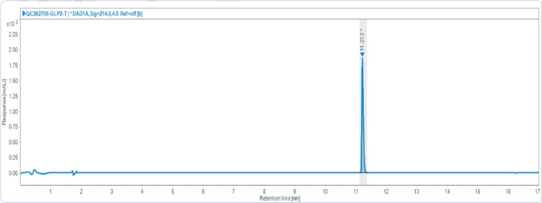
HPLC Chromatogram (Retention Time: 11.212 min)
