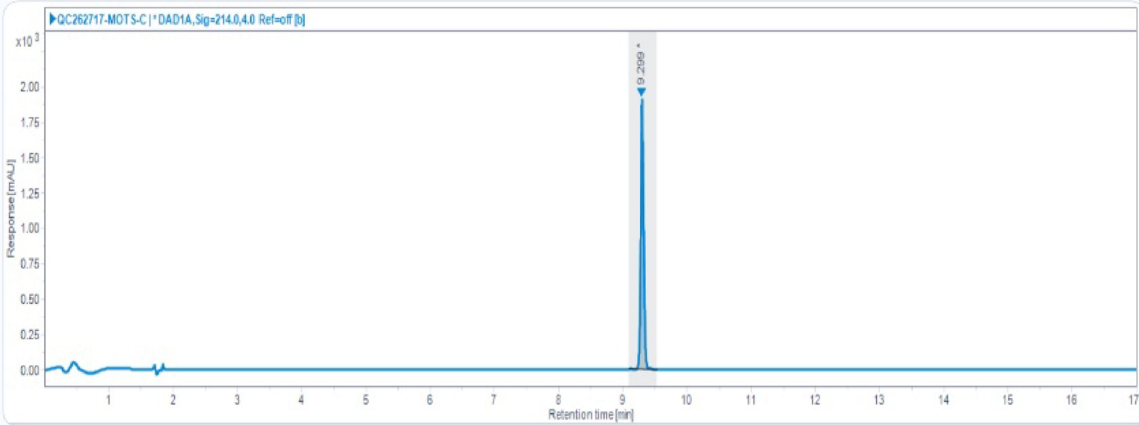
HPLC Chromatogram (Retention Time: 9.299 min)
