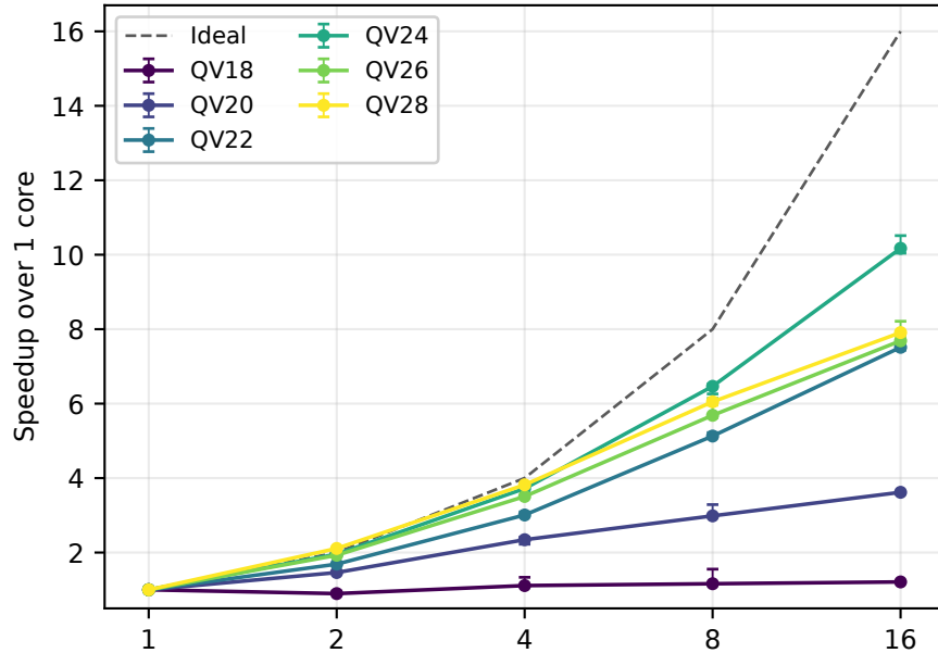
(b) Clifft 0.9.0 strong scaling
