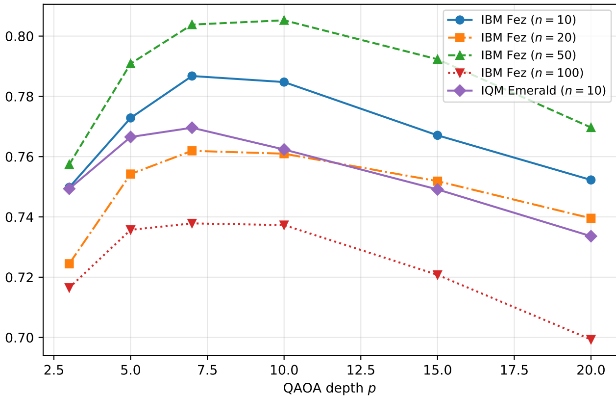
Approximation ratio
