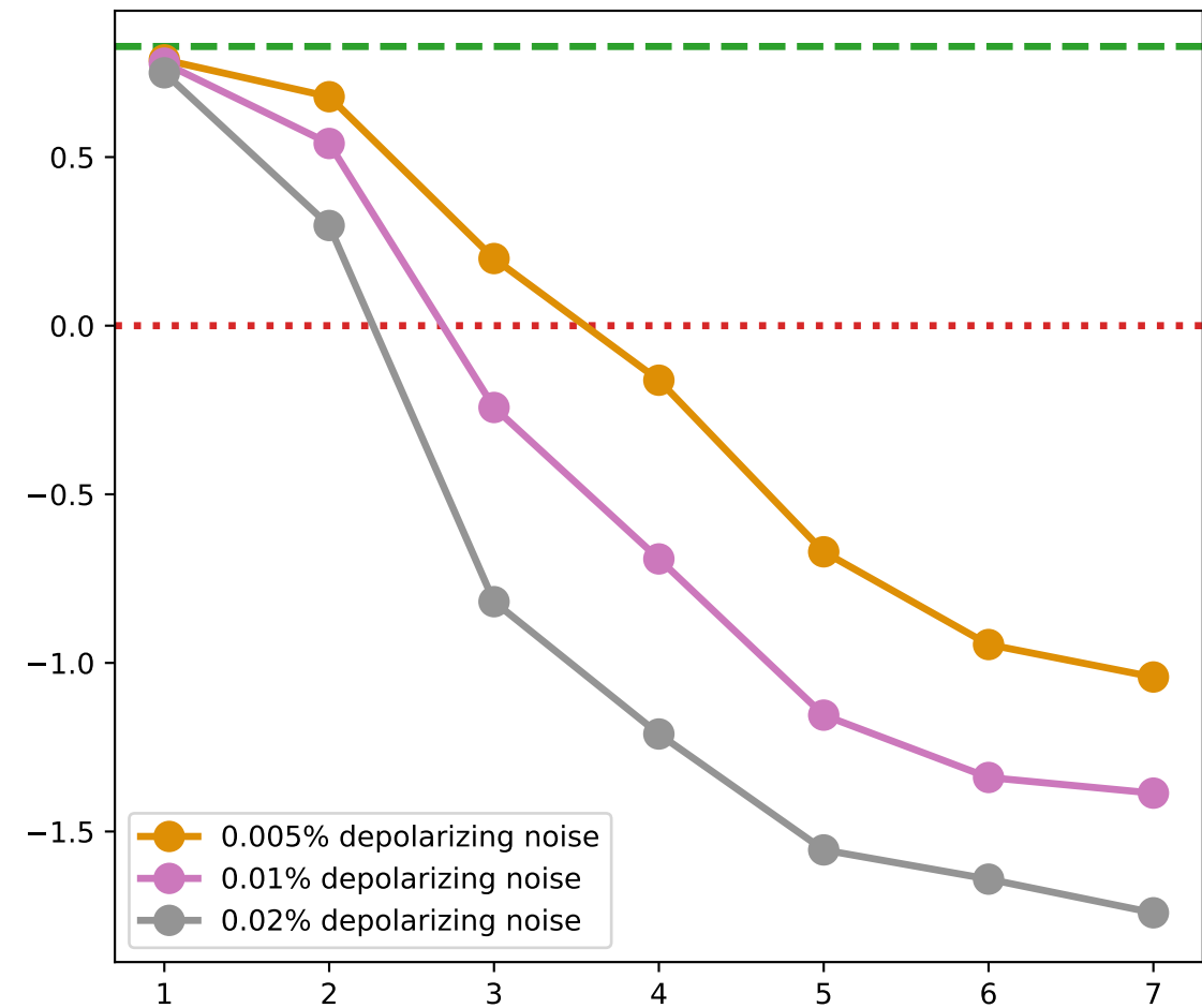
Dicke states
