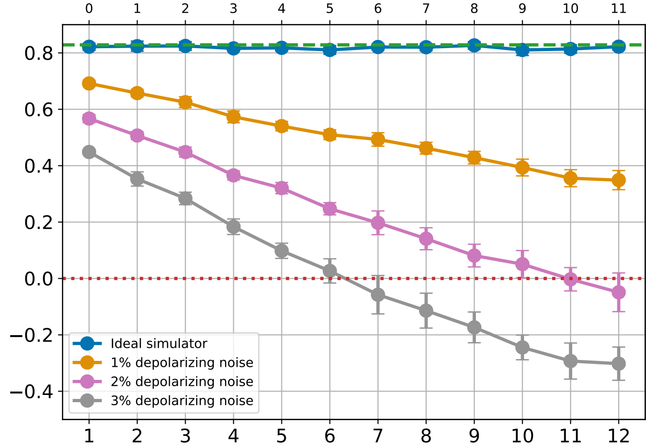
Random strategy
