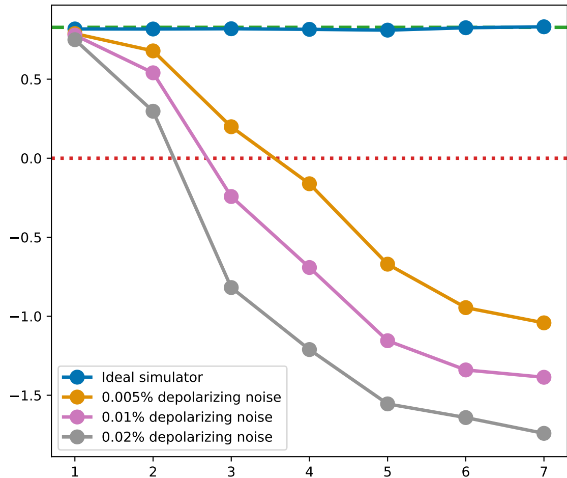
Dicke states
