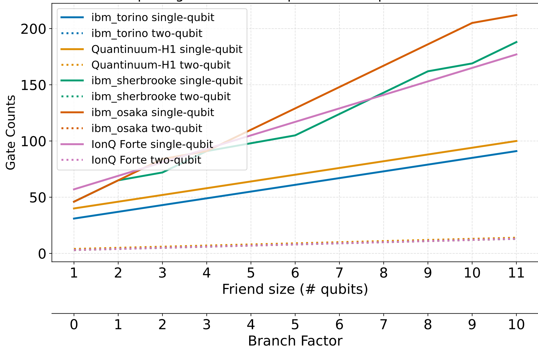
Compiled gate counts on quantum computer backends
