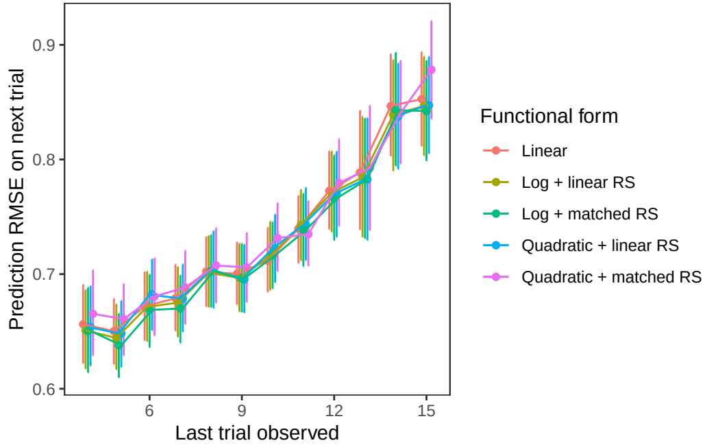
Figure 4: RMSE values for models with log LT and trial type interaction, plotted by the last trial observed in the model. Note that the x-axis begins at 4 (the minimum number of trials needed to support the number of parameters in quadratic models), and ends at 15 (one less than the maximum number of trials in the data). Error bars indicate bootstrapped 95% confidence intervals. RS: random slopes.
