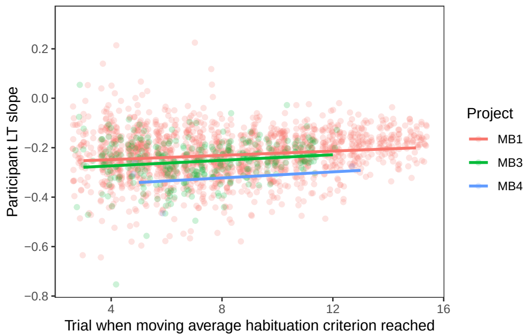
Figure 6: LT slopes for all participants by trial at which habituation criterion is reached. Lines indicate best-fitting linear regressions; confidence bands were excluded due to visual clutter.
