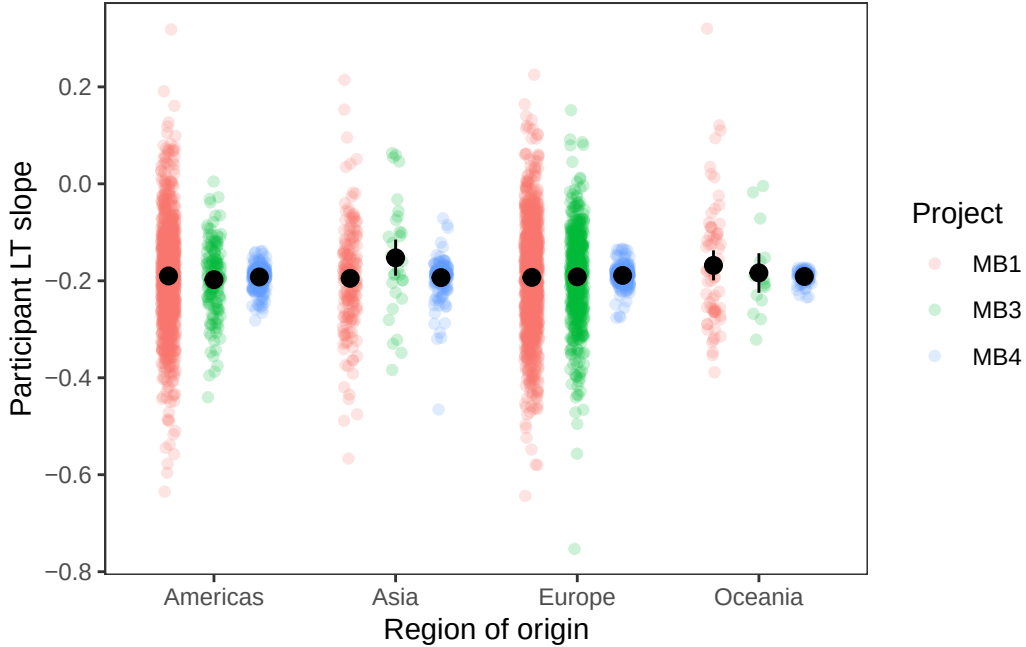
Figure 8: LT slopes for all participants by region of origin. Black dots and error bars indicate group means and bootstrapped 95% confidence intervals.
