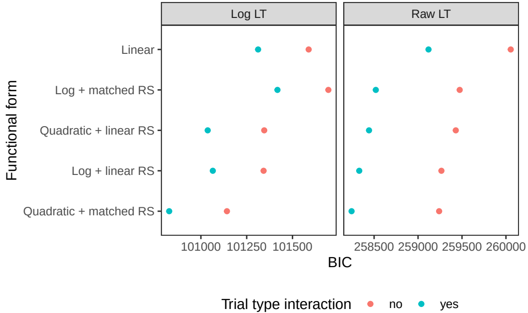
Figure 3: BIC values for all models tested, faceted by outcome transformation. Note that the x-axis values differ across the two facets. RS: random slopes.
