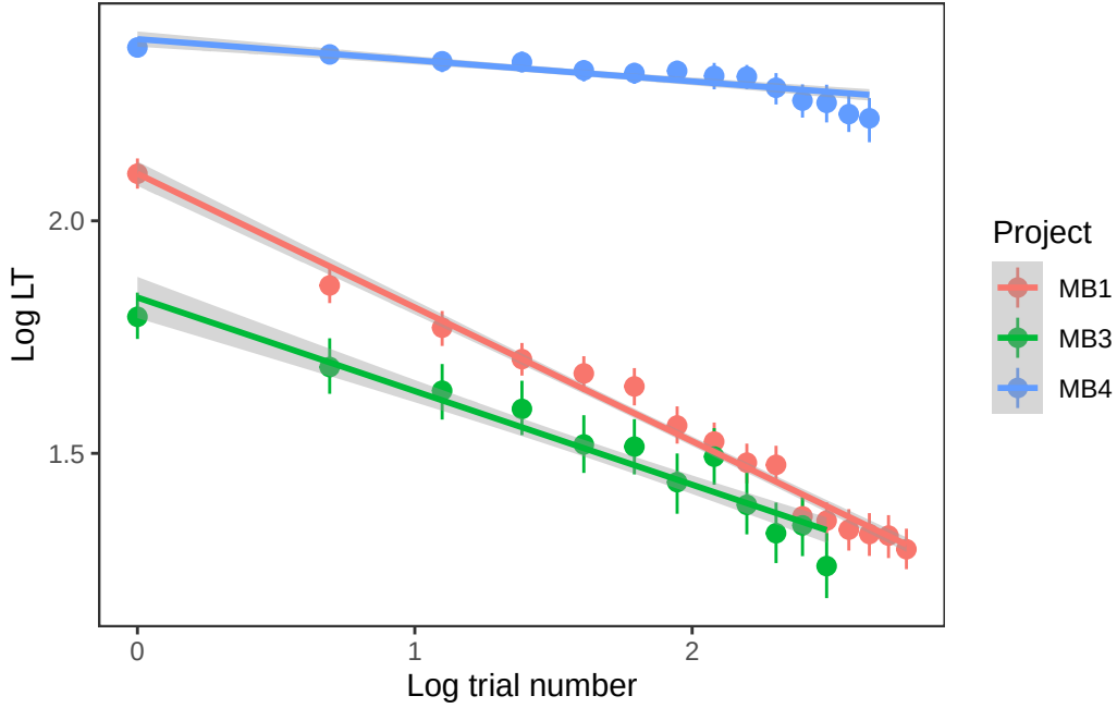
Figure 2: Log LT by log trial number. Points and error bars indicate all-participant means and bootstrapped 95% confidence intervals. Lines and shaded bands indicate best-fitting linear regressions and their 95% confidence bands.
