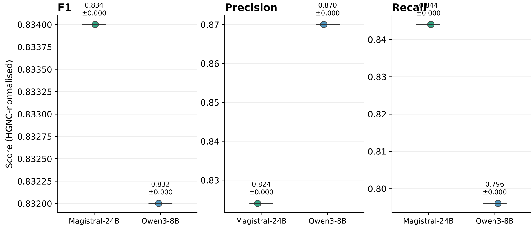
Run-to-run variation, prompt v6, three independent seeds — 267-paper OATargets set
