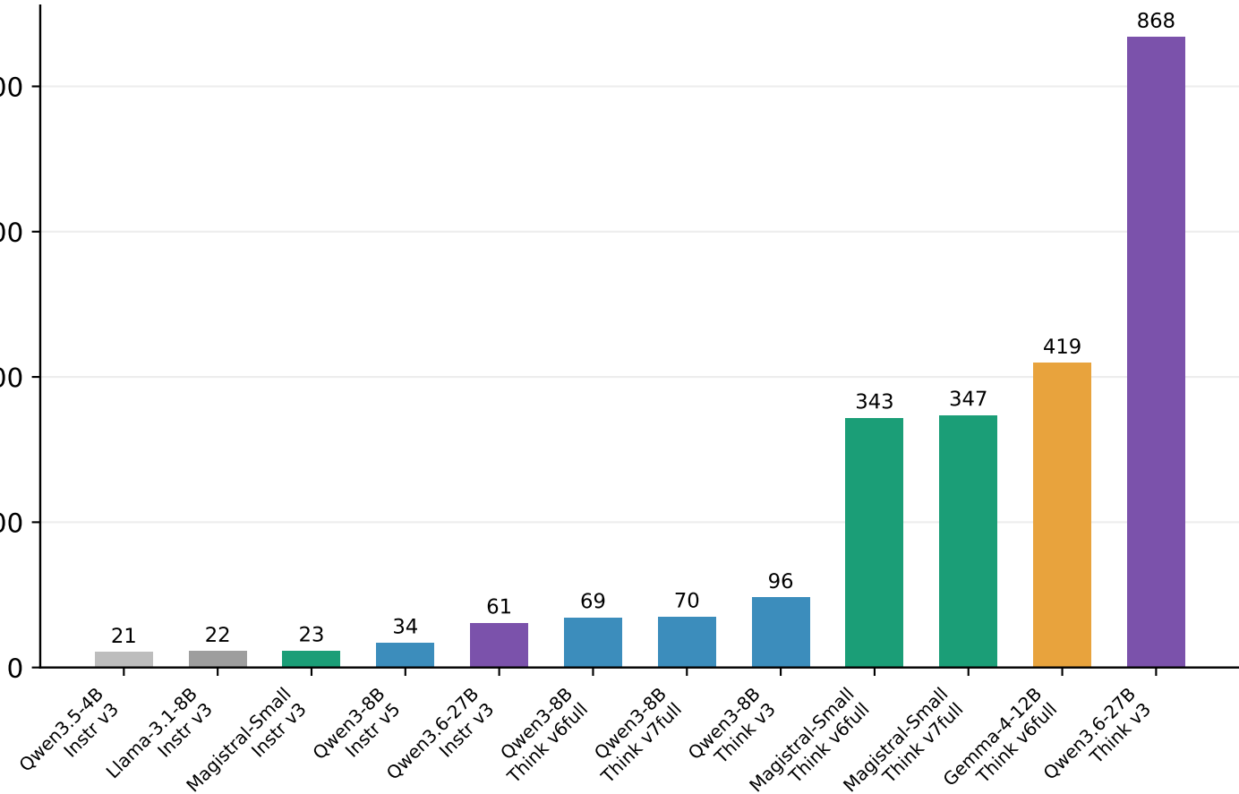
Projected GPU-hours for 11,000 abstracts
