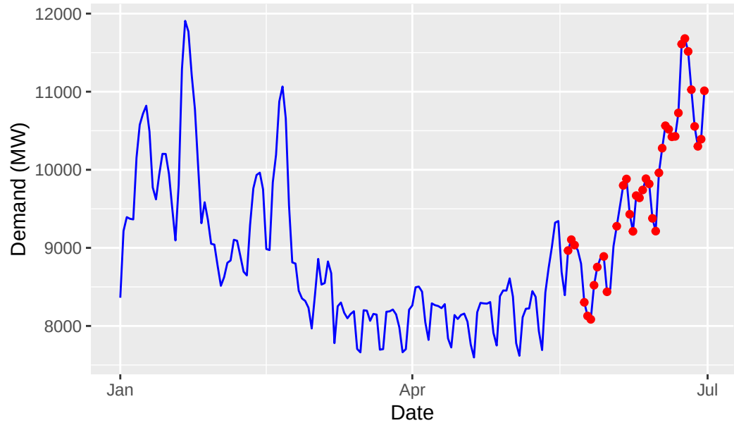
Daily Electricity Demand with High Water Temperature Days
