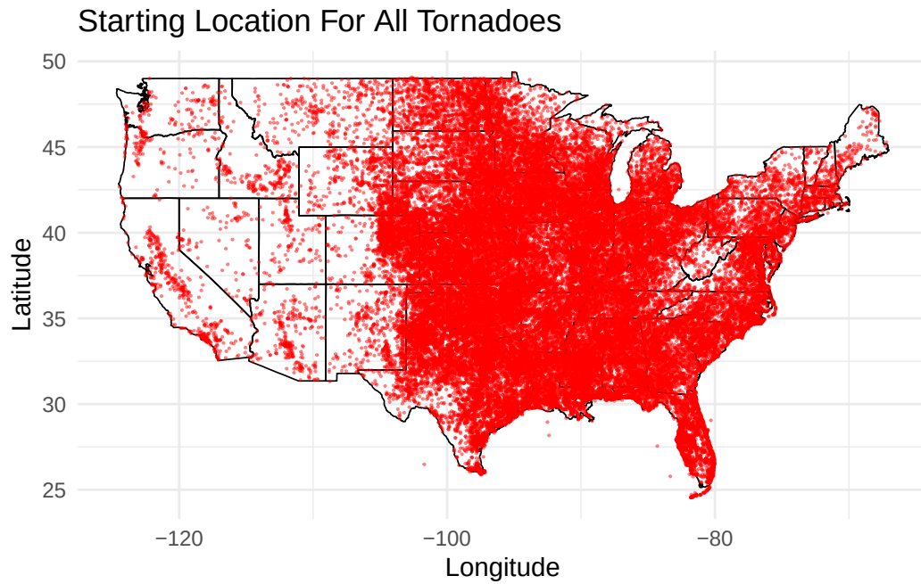
Figure 4.2: Starting locations of all tornadoes in the continental United States.
