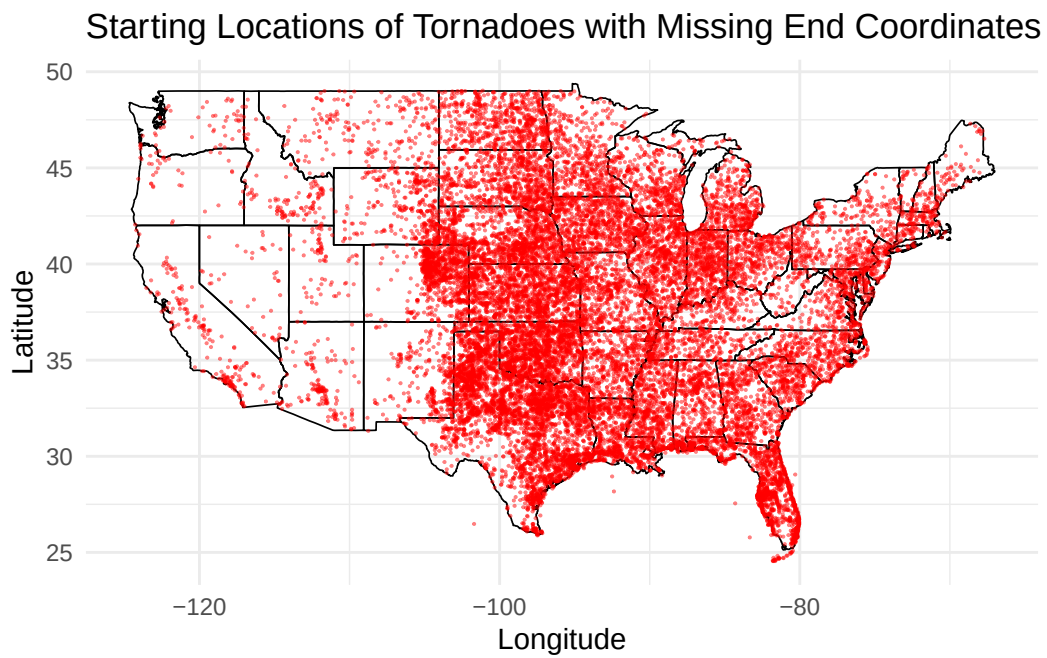
Figure 4.3: Starting locations of tornadoes with missing end coordinates.
