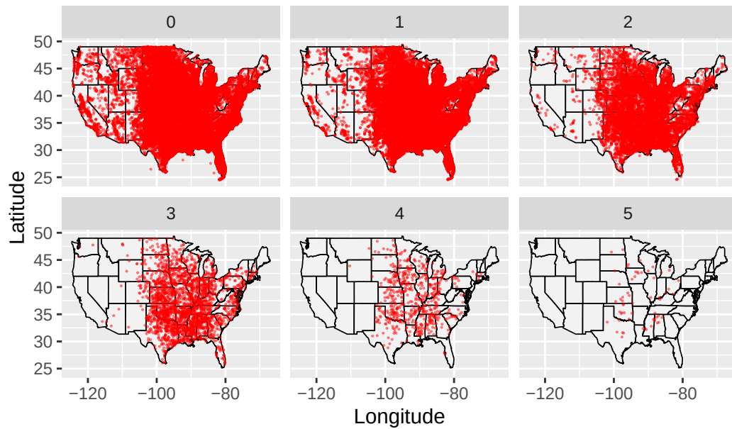
Figure 4.4: Starting locations of all tornadoes in the continental United States grouped by magnitude on EF scale
