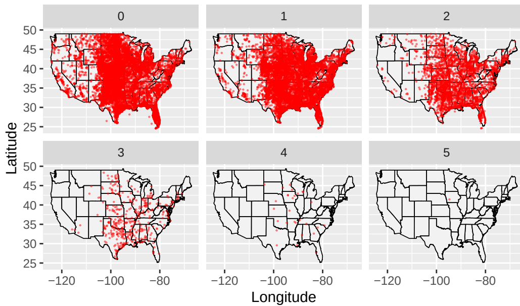
Figure 4.5: Starting locations of tornadoes with missing end coordinates grouped by magnitude on EF scale
