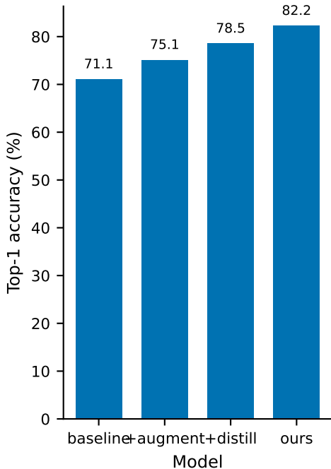
(a) CIFAR-10
