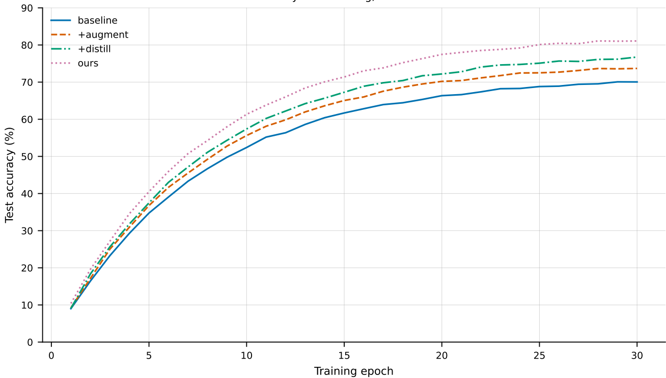
Accuracy over training, double column
